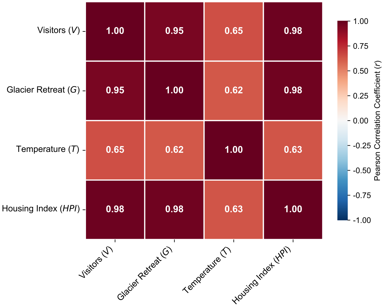
Correlation Matrix of Key Variables
